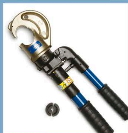
Pressa idraulica da 13 ton. Hydraulic press power 13 tons.
